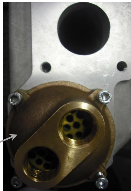
Fig 2n Wasting anode
